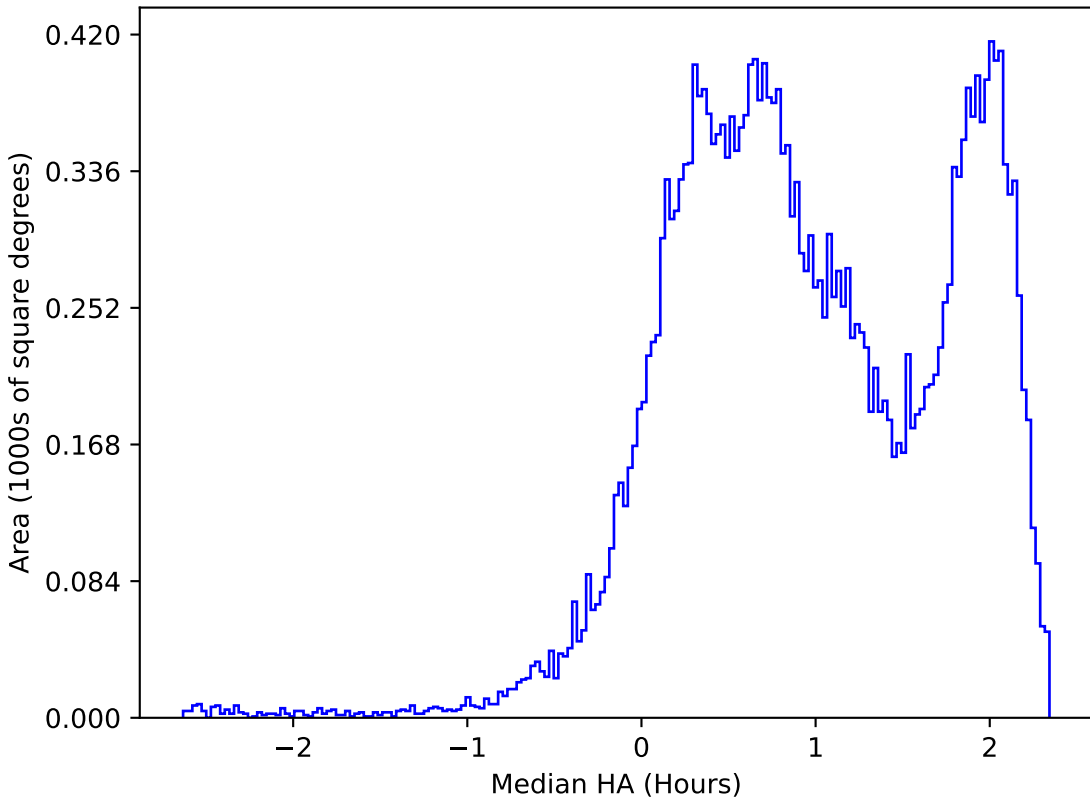
too_elab_r16_d3_gz_v3.4_10yrs All sky i band: Median HA
