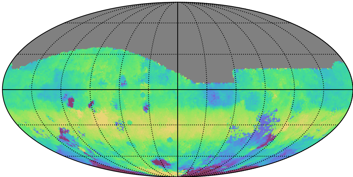
too_elab_r16_d3_gz_v3.4_10yrs All sky g band: Median HA
