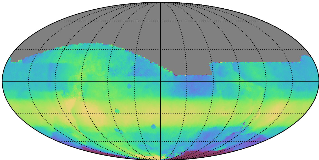
too_elab_r16_d3_gz_v3.4_10yrs All sky all bands: Median HA
