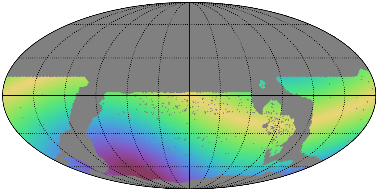
too_elab_r16_d3_gz_v3.4_10yrs WFD z band: Max solarElong
