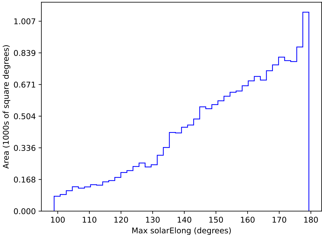
too_elab_r16_d3_gz_v3.4_10yrs WFD z band: Max solarElong
