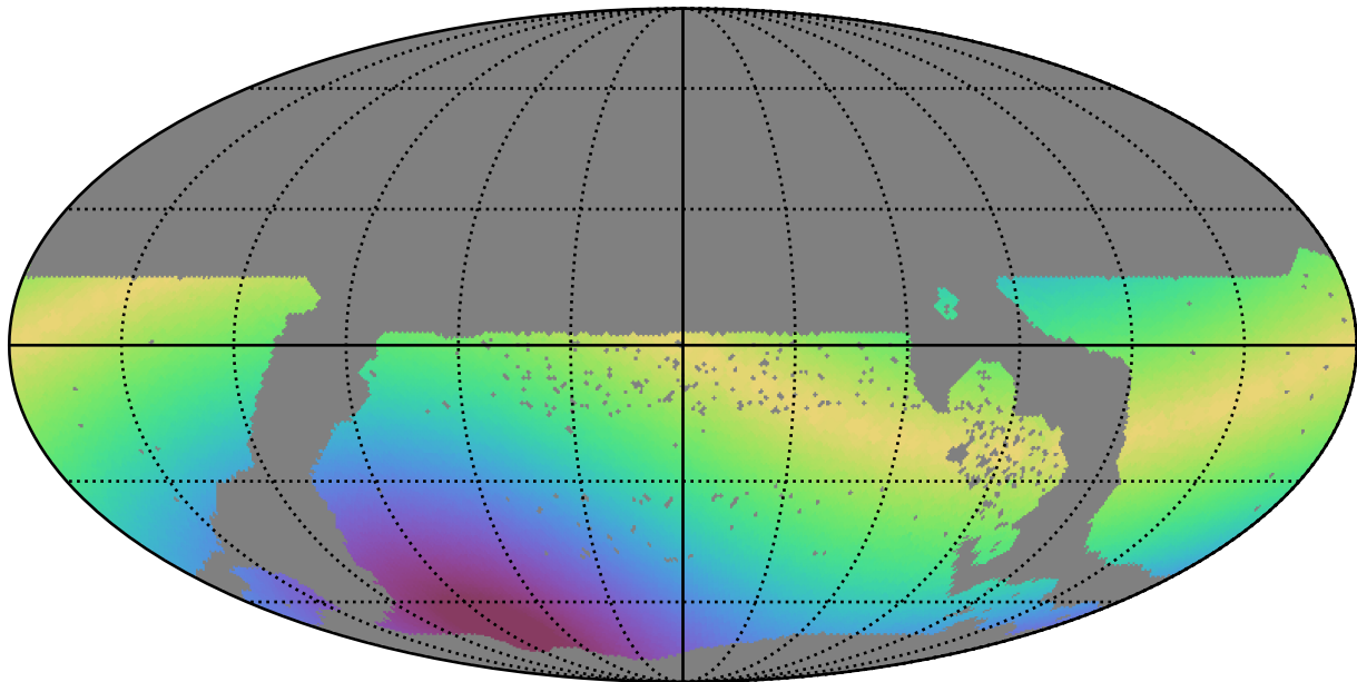
too_elab_r16_d3_gz_v3.4_10yrs WFD y band: Max solarElong
