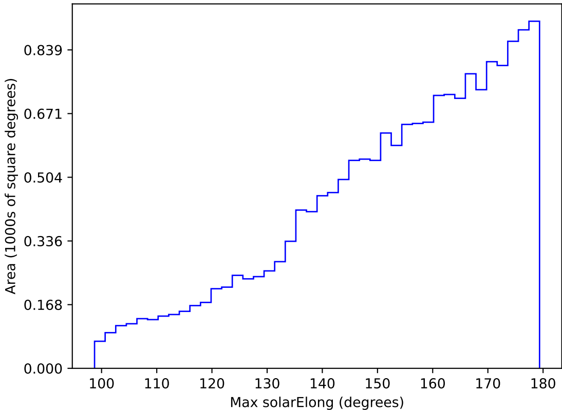
too_elab_r16_d3_gz_v3.4_10yrs WFD y band: Max solarElong
