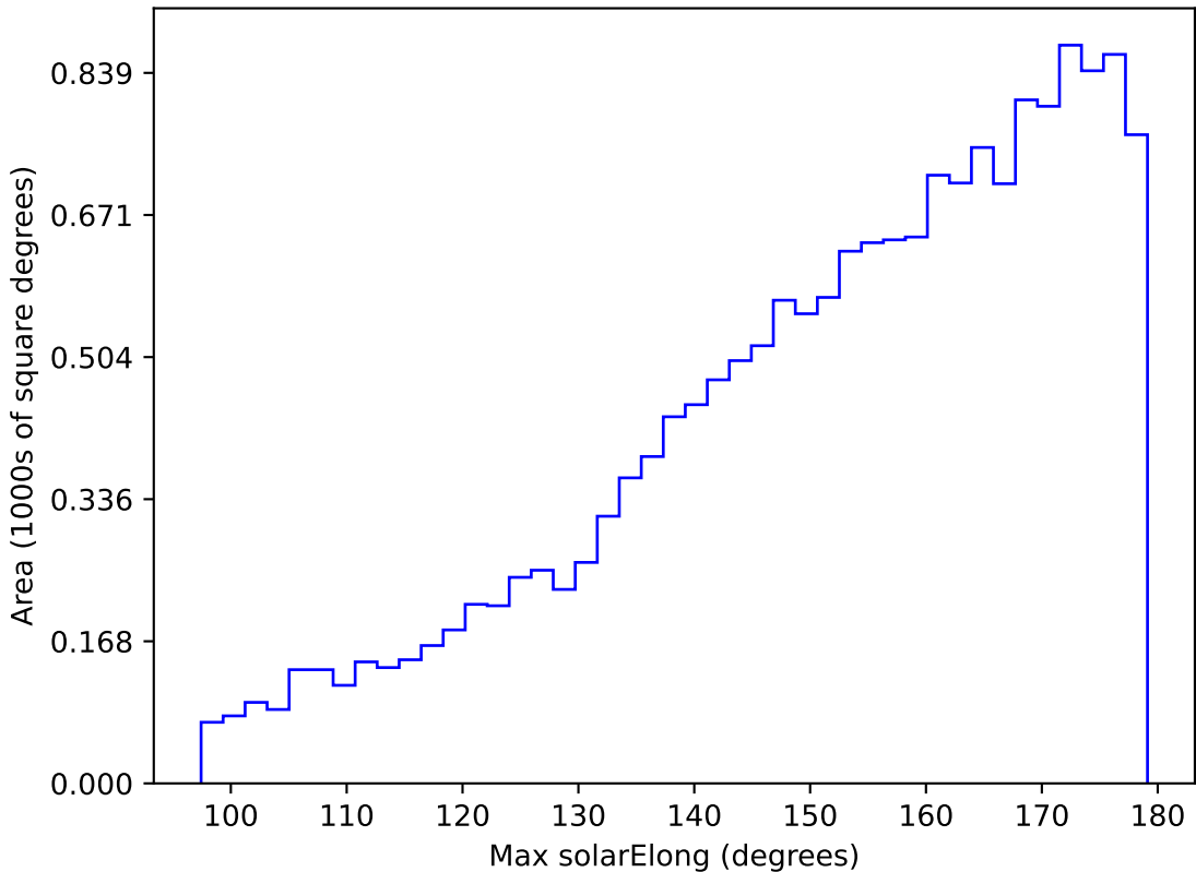
too_elab_r16_d3_gz_v3.4_10yrs WFD u band: Max solarElong
