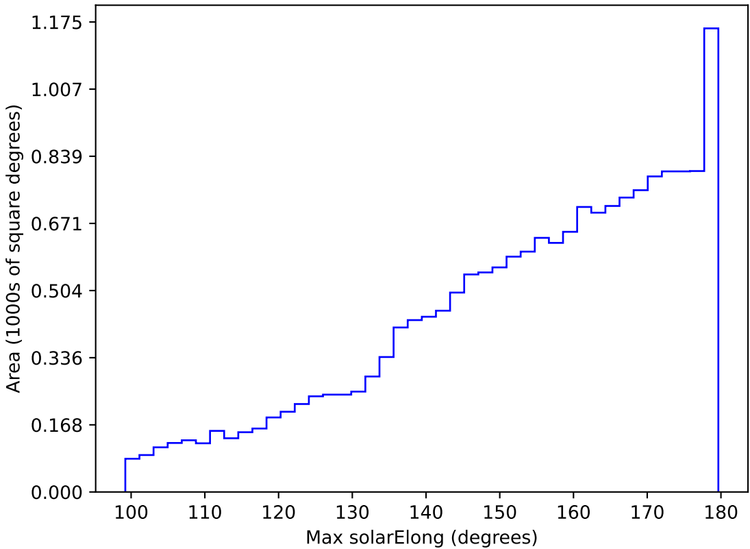
too_elab_r16_d3_gz_v3.4_10yrs WFD all bands: Max solarElong
