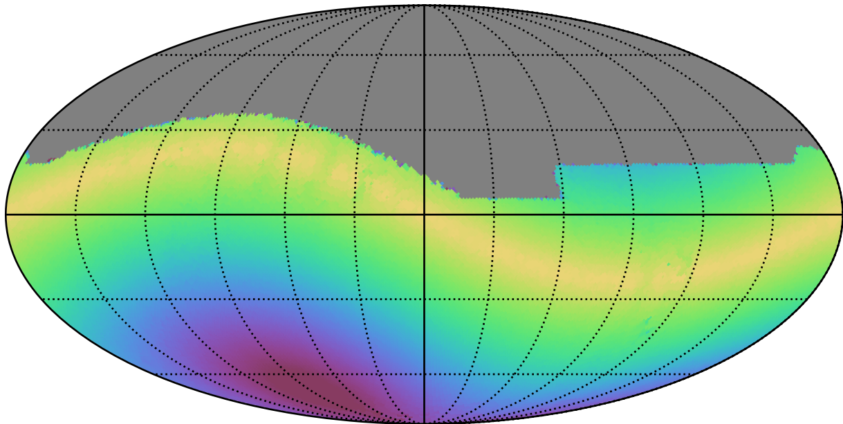
too_elab_r16_d3_gz_v3.4_10yrs All sky z band: Max solarElong
