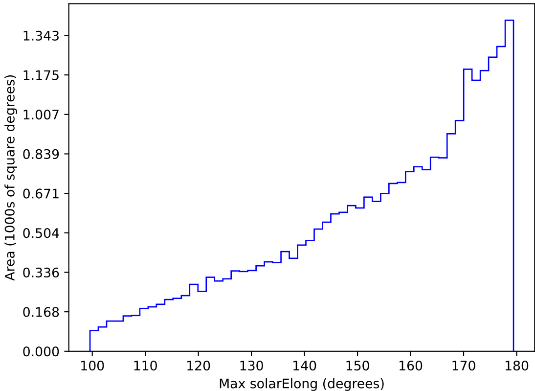
too_elab_r16_d3_gz_v3.4_10yrs All sky r band: Max solarElong
