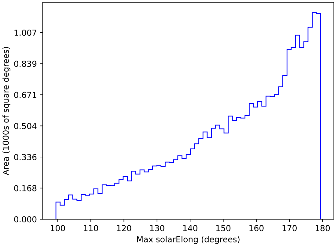
too_elab_r16_d3_gz_v3.4_10yrs All sky i band: Max solarElong
