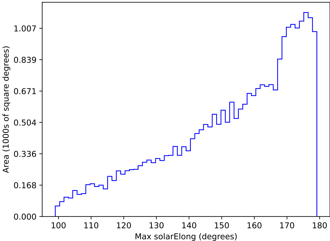
too_elab_r16_d3_gz_v3.4_10yrs All sky g band: Max solarElong
