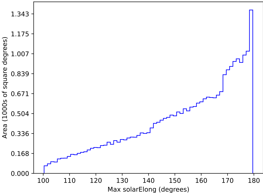
too_elab_r16_d3_gz_v3.4_10yrs All sky all bands: Max solarElong
