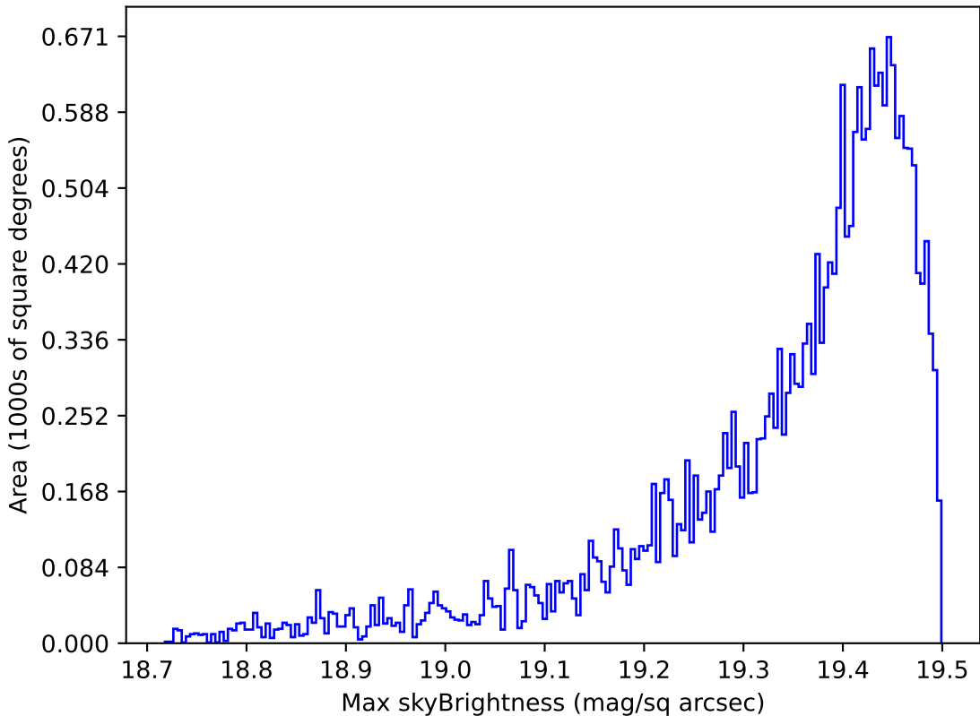
too_elab_r16_d3_gz_v3.4_10yrs Yr 1 z band: Max skyBrightness
