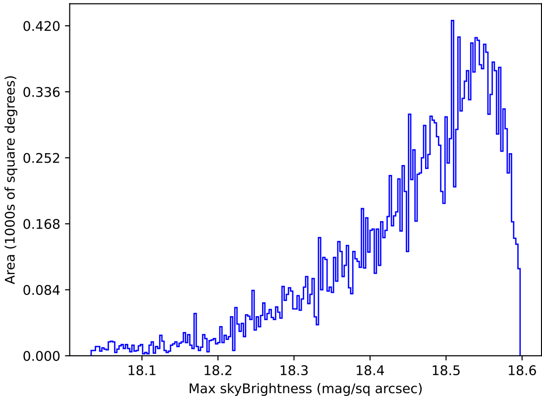
too_elab_r16_d3_gz_v3.4_10yrs Yr 1 y band: Max skyBrightness
