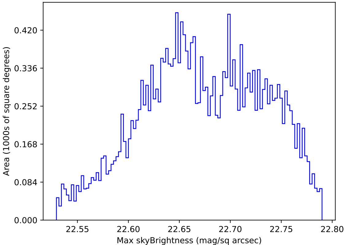
too_elab_r16_d3_gz_v3.4_10yrs Yr 1 u band: Max skyBrightness
