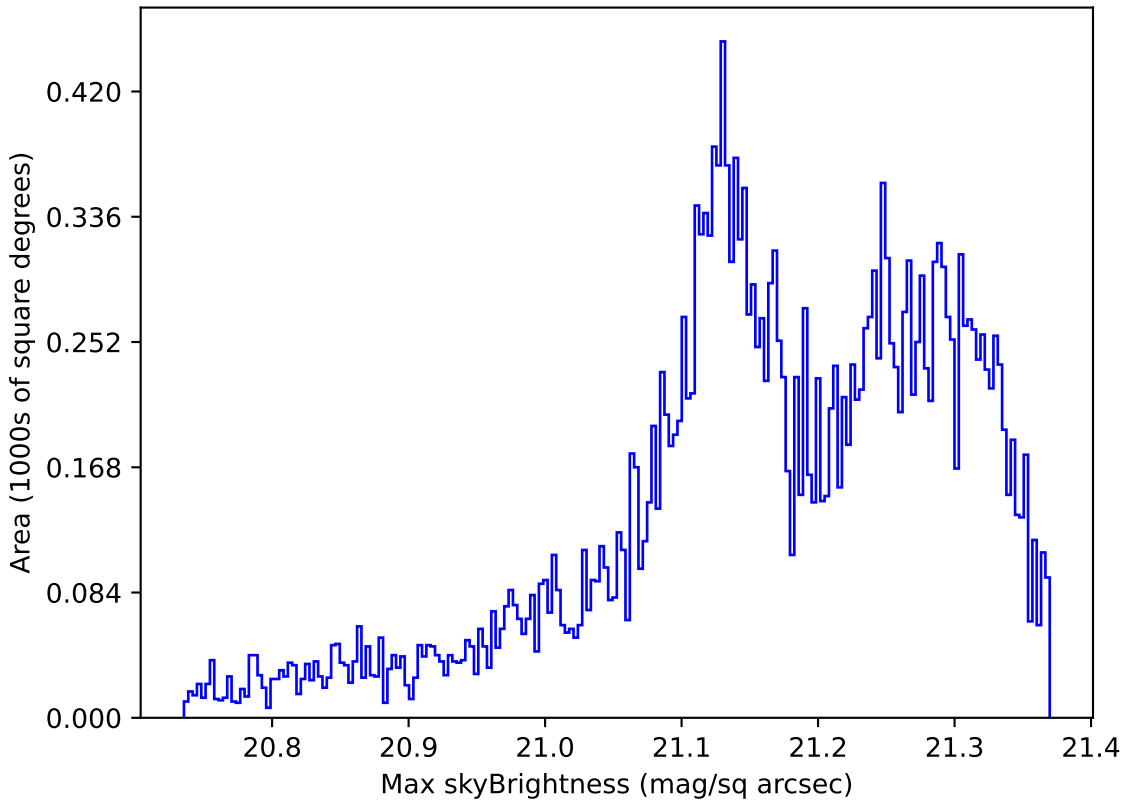
too_elab_r16_d3_gz_v3.4_10yrs Yr 1 r band: Max skyBrightness
