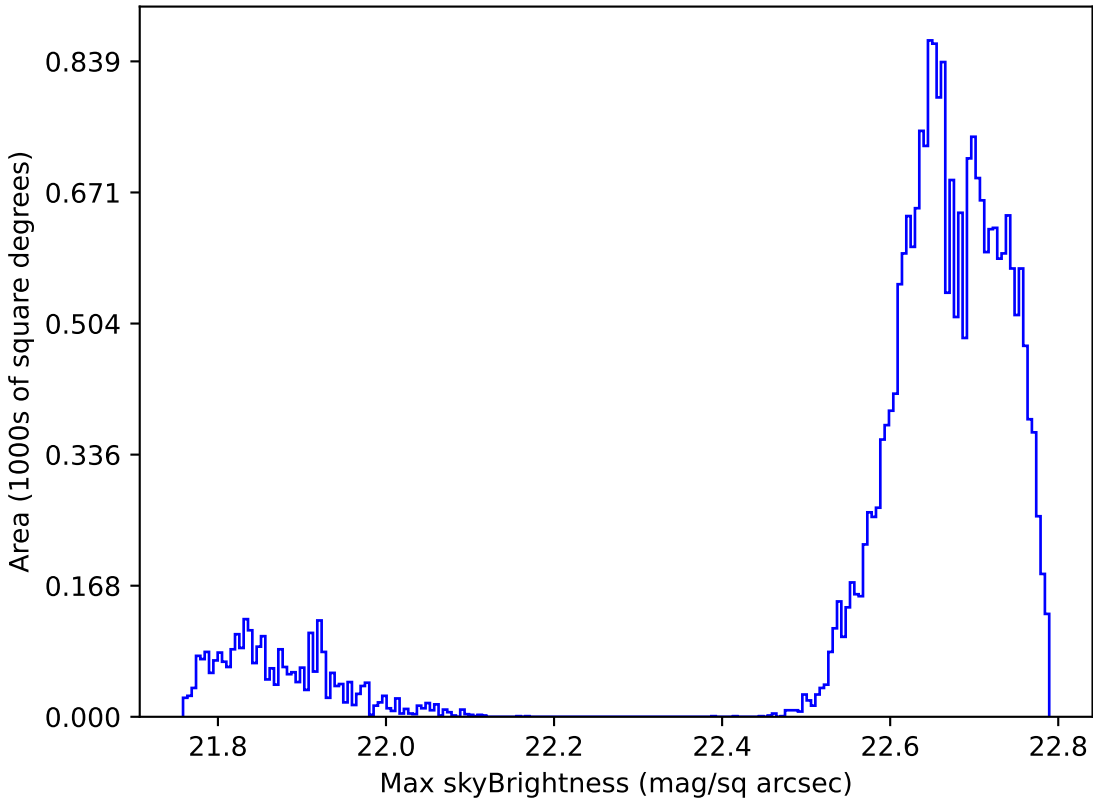
too_elab_r16_d3_gz_v3.4_10yrs Yr 1 all bands: Max skyBrightness
