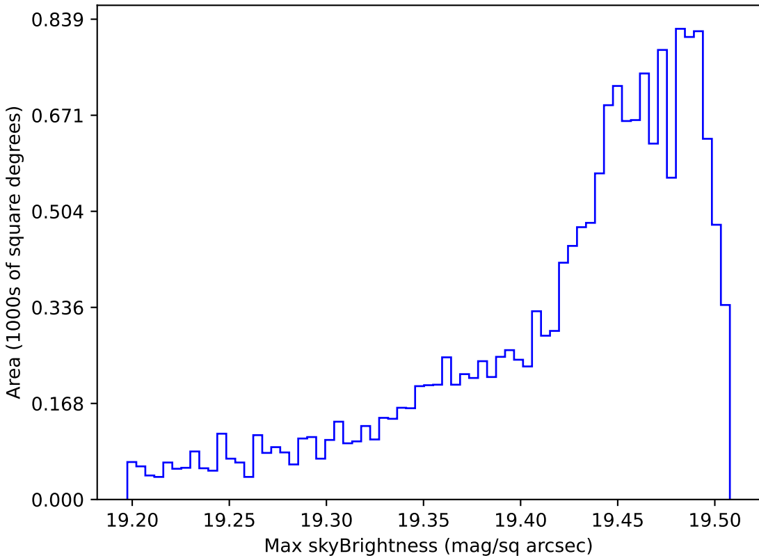
too_elab_r16_d3_gz_v3.4_10yrs WFD z band: Max skyBrightness
