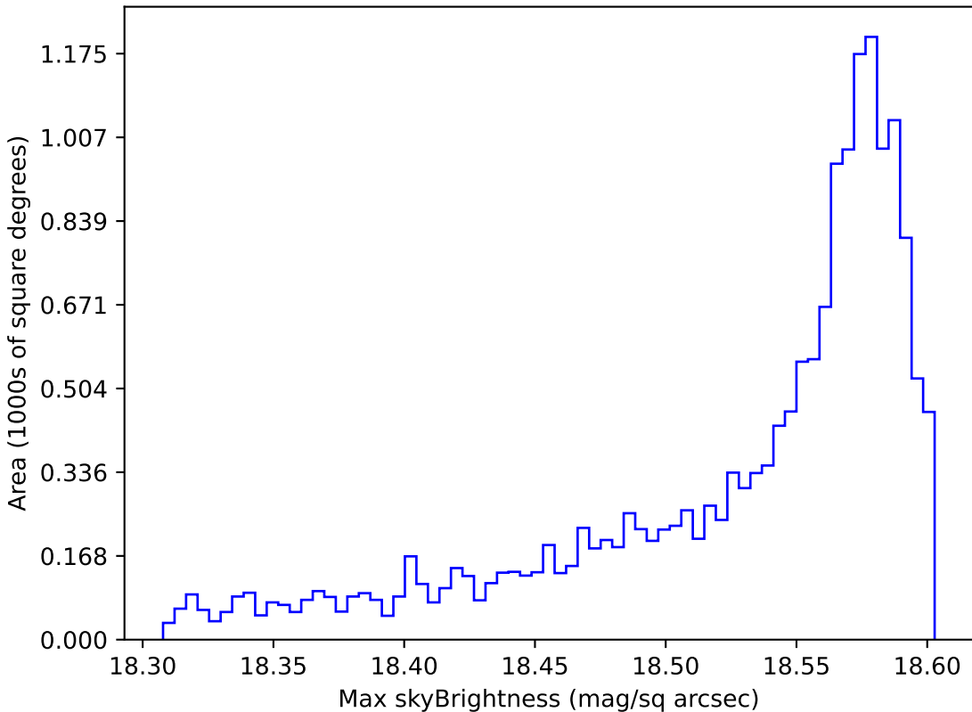
too_elab_r16_d3_gz_v3.4_10yrs WFD y band: Max skyBrightness
