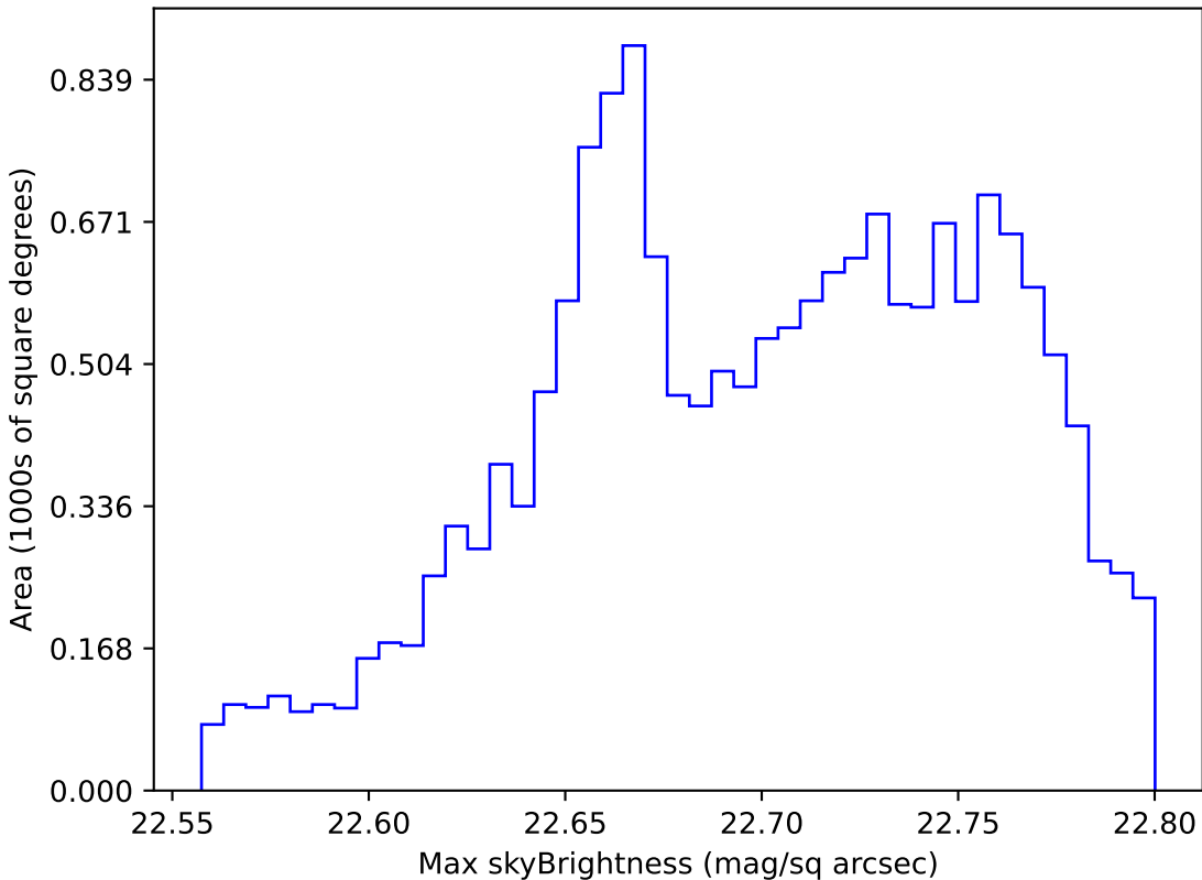
too_elab_r16_d3_gz_v3.4_10yrs WFD u band: Max skyBrightness
