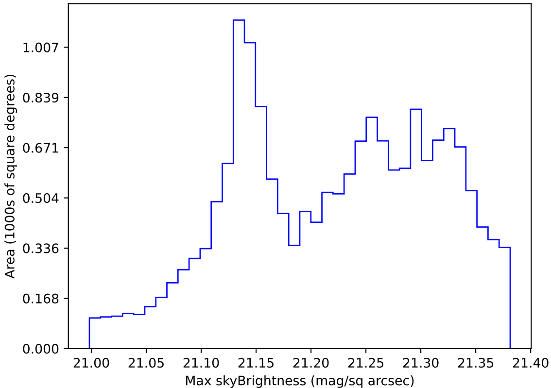
too_elab_r16_d3_gz_v3.4_10yrs WFD r band: Max skyBrightness
