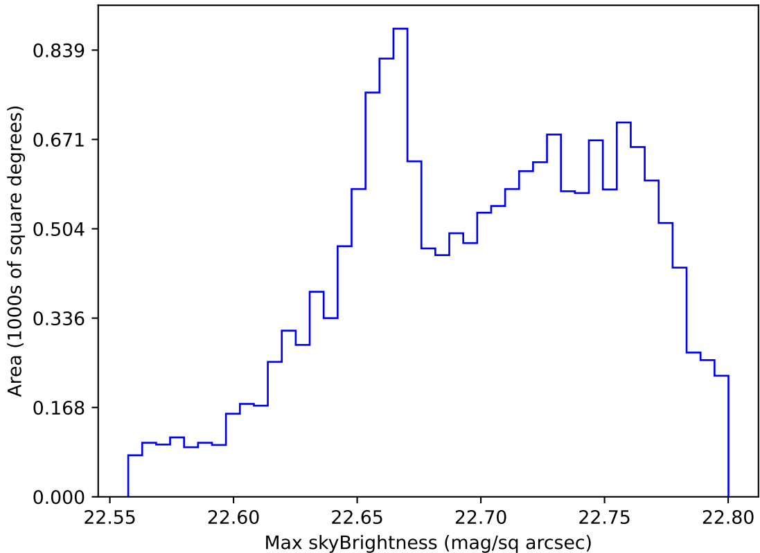
too_elab_r16_d3_gz_v3.4_10yrs WFD all bands: Max skyBrightness
