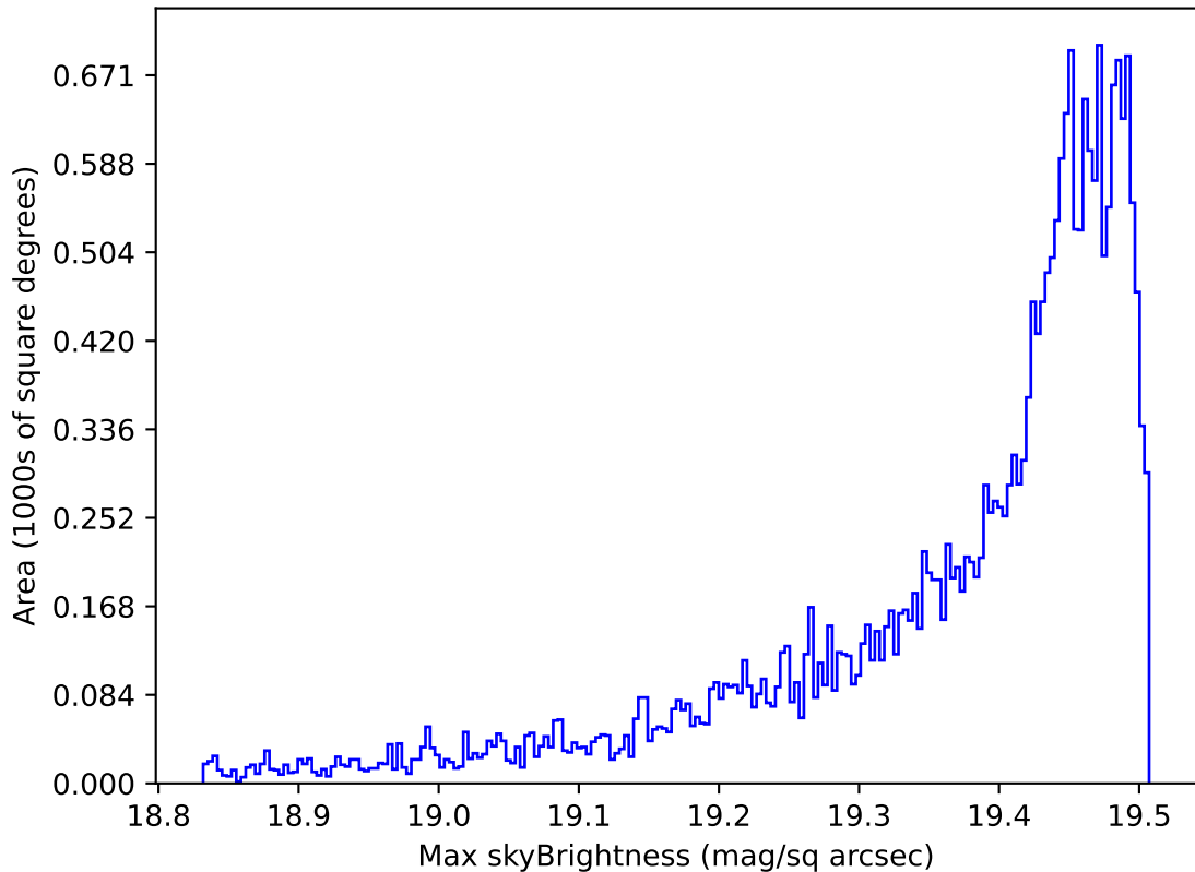
too_elab_r16_d3_gz_v3.4_10yrs All sky z band: Max skyBrightness
