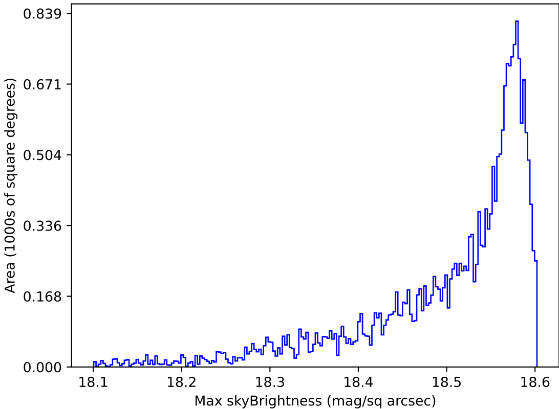
too_elab_r16_d3_gz_v3.4_10yrs All sky y band: Max skyBrightness
