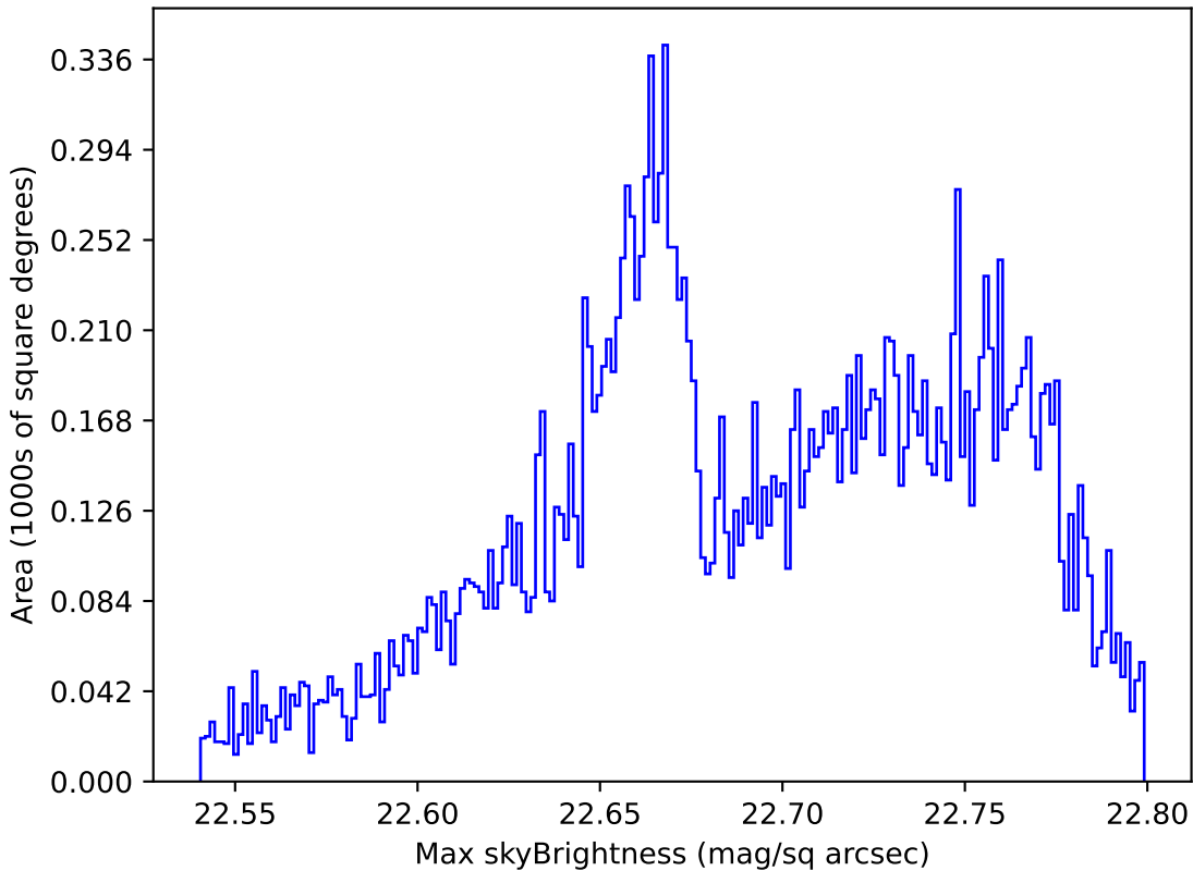
too_elab_r16_d3_gz_v3.4_10yrs All sky u band: Max skyBrightness
