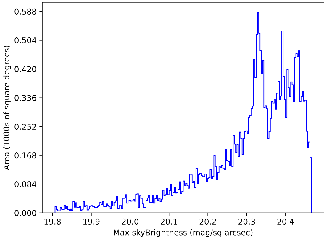
too_elab_r16_d3_gz_v3.4_10yrs All sky i band: Max skyBrightness
