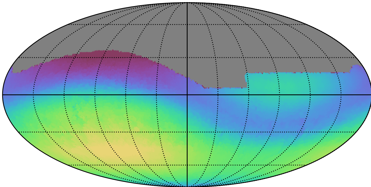
too_elab_r16_d3_gz_v3.4_10yrs All sky g band: Max skyBrightness
