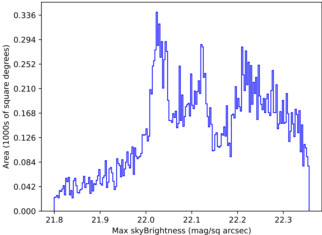
too_elab_r16_d3_gz_v3.4_10yrs All sky g band: Max skyBrightness
