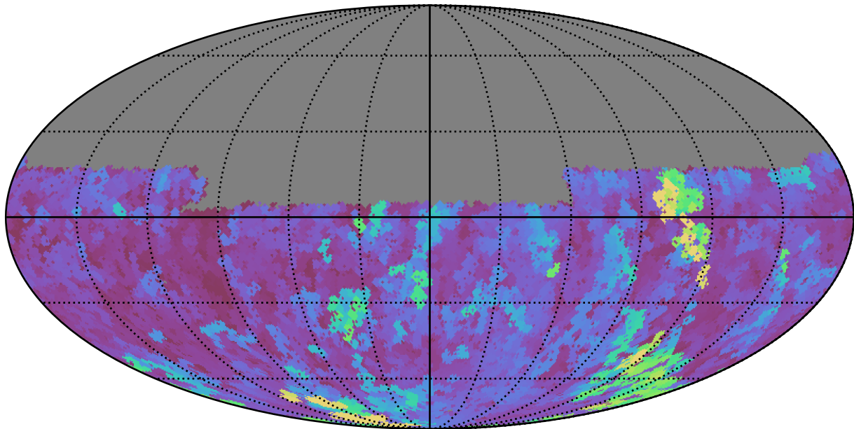
too_elab_r16_d3_gz_v3.4_10yrs Yr 1 u band: Max seeingGeom
