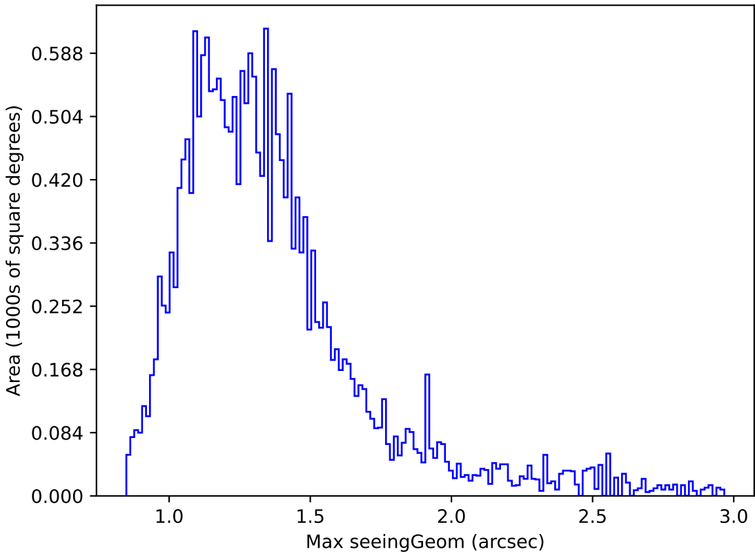
too_elab_r16_d3_gz_v3.4_10yrs Yr 1 u band: Max seeingGeom
