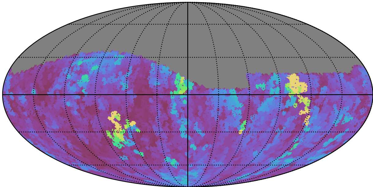
too_elab_r16_d3_gz_v3.4_10yrs Yr 1 g band: Max seeingGeom
