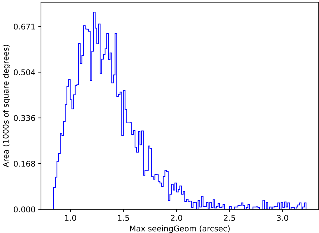
too_elab_r16_d3_gz_v3.4_10yrs Yr 1 g band: Max seeingGeom
