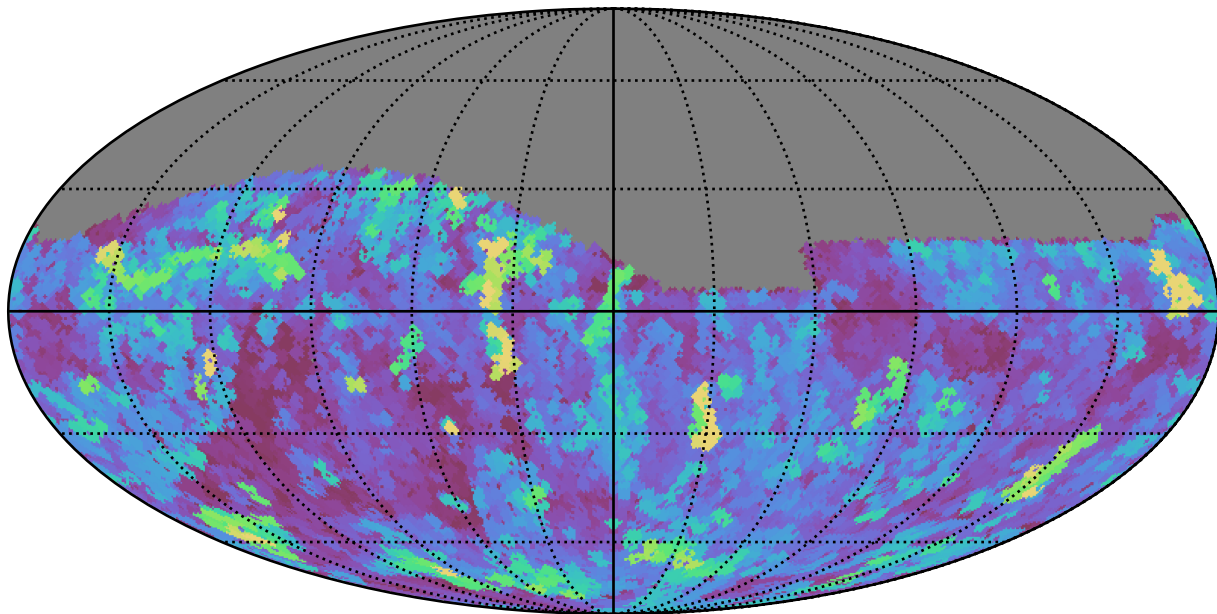
too_elab_r16_d3_gz_v3.4_10yrs Yr 1 z band: Max seeingEff
