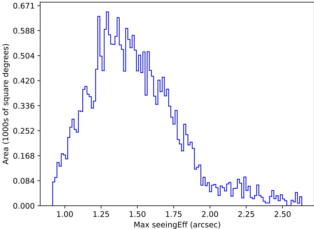
too_elab_r16_d3_gz_v3.4_10yrs Yr 1 z band: Max seeingEff
