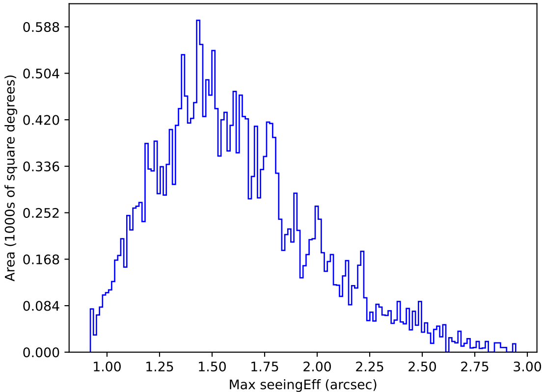
too_elab_r16_d3_gz_v3.4_10yrs Yr 1 r band: Max seeingEff
