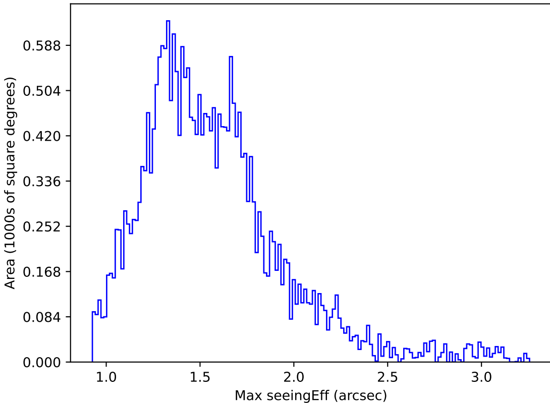
too_elab_r16_d3_gz_v3.4_10yrs Yr 1 i band: Max seeingEff
