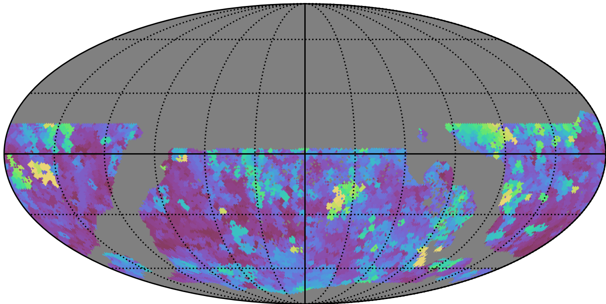
too_elab_r16_d3_gz_v3.4_10yrs WFD i band: Max seeingEff
