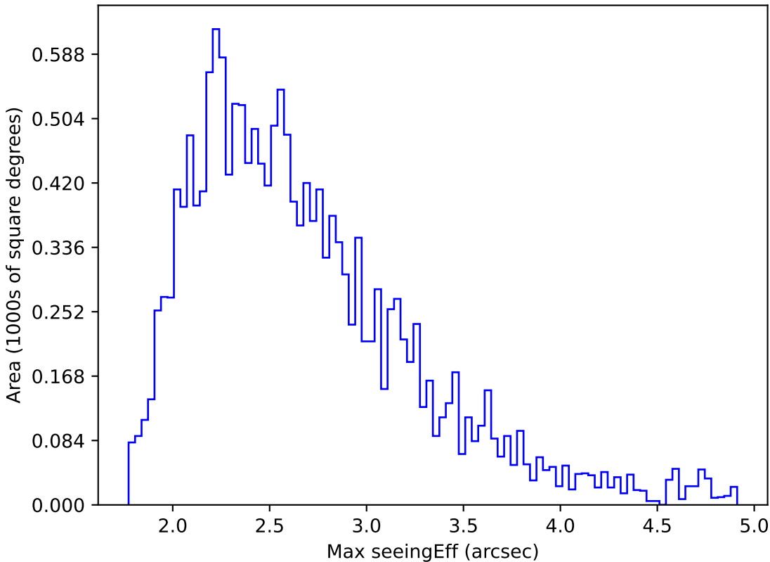
too_elab_r16_d3_gz_v3.4_10yrs WFD i band: Max seeingEff
