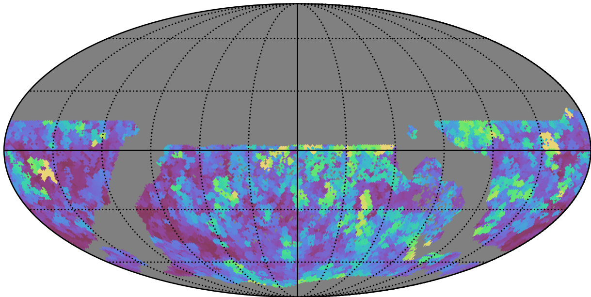
too_elab_r16_d3_gz_v3.4_10yrs WFD all bands: Max seeingEff
