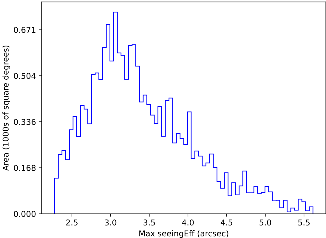
too_elab_r16_d3_gz_v3.4_10yrs WFD all bands: Max seeingEff
