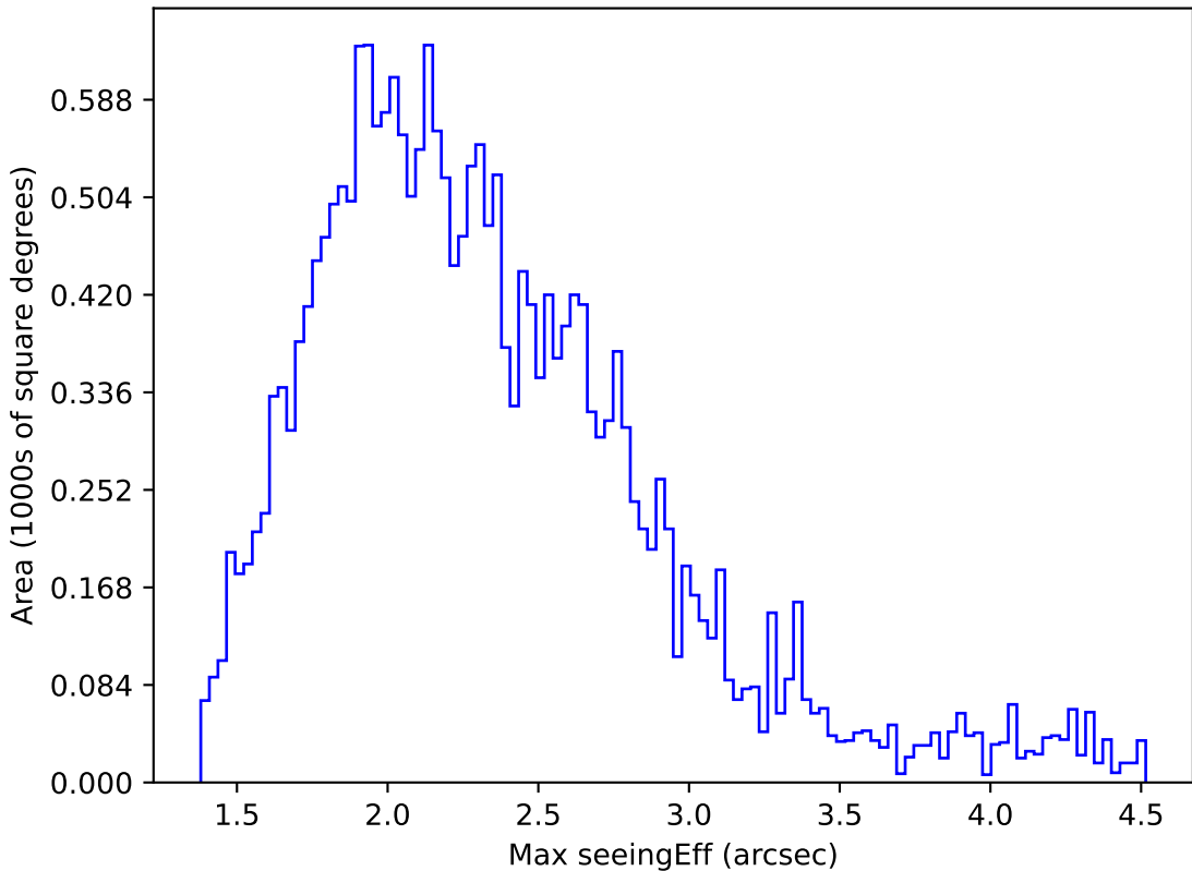
too_elab_r16_d3_gz_v3.4_10yrs All sky y band: Max seeingEff
