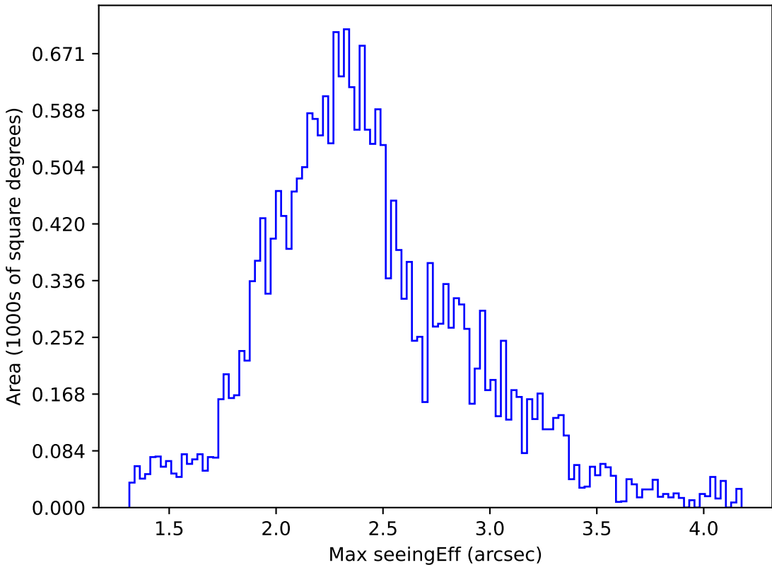
too_elab_r16_d3_gz_v3.4_10yrs All sky u band: Max seeingEff
