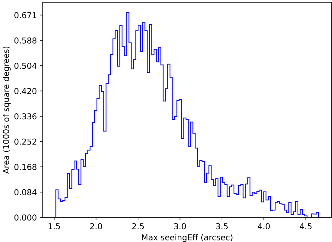
too_elab_r16_d3_gz_v3.4_10yrs All sky r band: Max seeingEff
