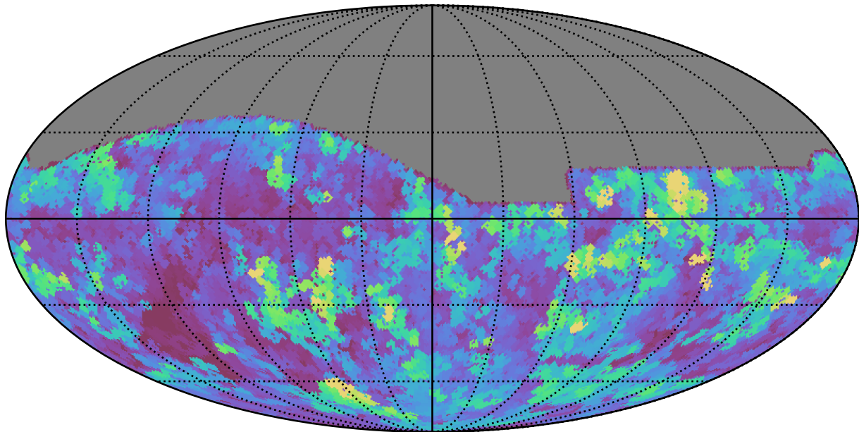
too_elab_r16_d3_gz_v3.4_10yrs All sky g band: Max seeingEff
