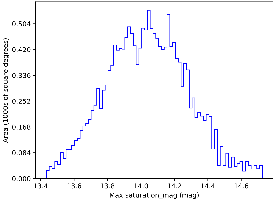
too_elab_r16_d3_gz_v3.4_10yrs WFD u band: Max saturation_mag
