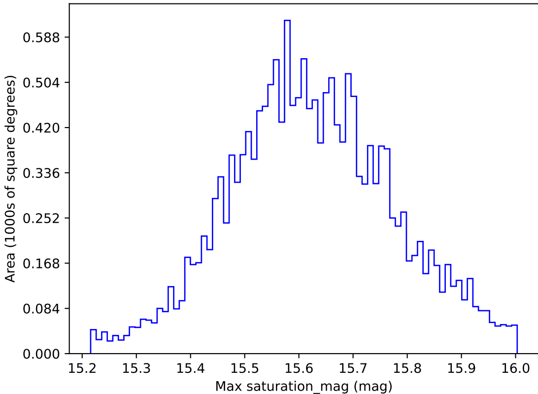
too_elab_r16_d3_gz_v3.4_10yrs WFD i band: Max saturation_mag
