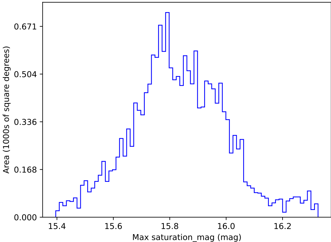
too_elab_r16_d3_gz_v3.4_10yrs WFD all bands: Max saturation_mag
