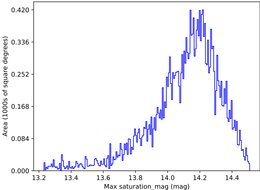
too_elab_r16_d3_gz_v3.4_10yrs All sky y band: Max saturation_mag
